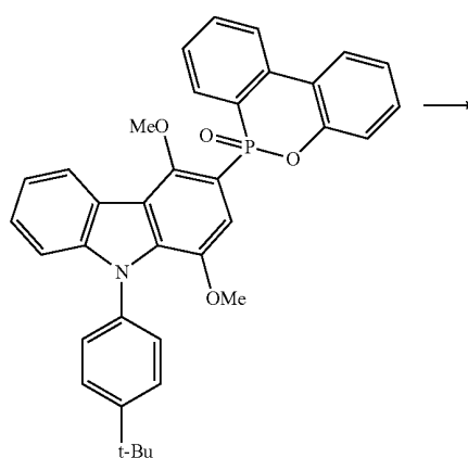
Compound 201
